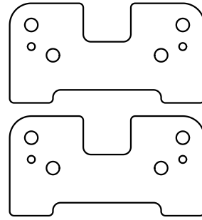
#2: X support block
